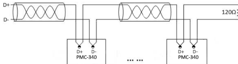
Figure 2-7 RS-485 Connections
